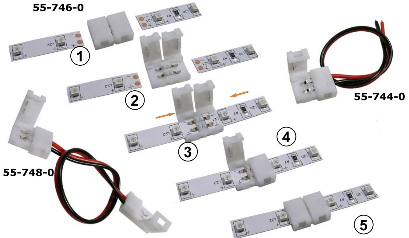
Snap-on LED Strip Connectors
