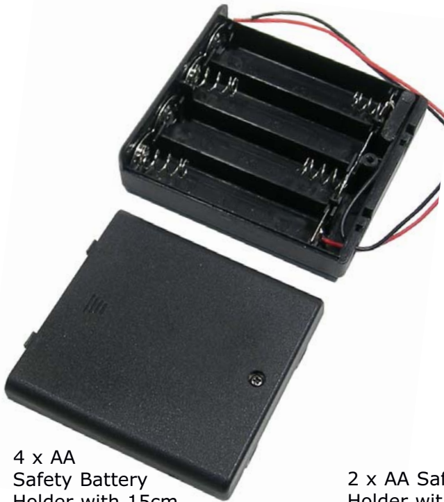
4 x AA Battery Holder with 15cm UL1007 26AWG Wire
